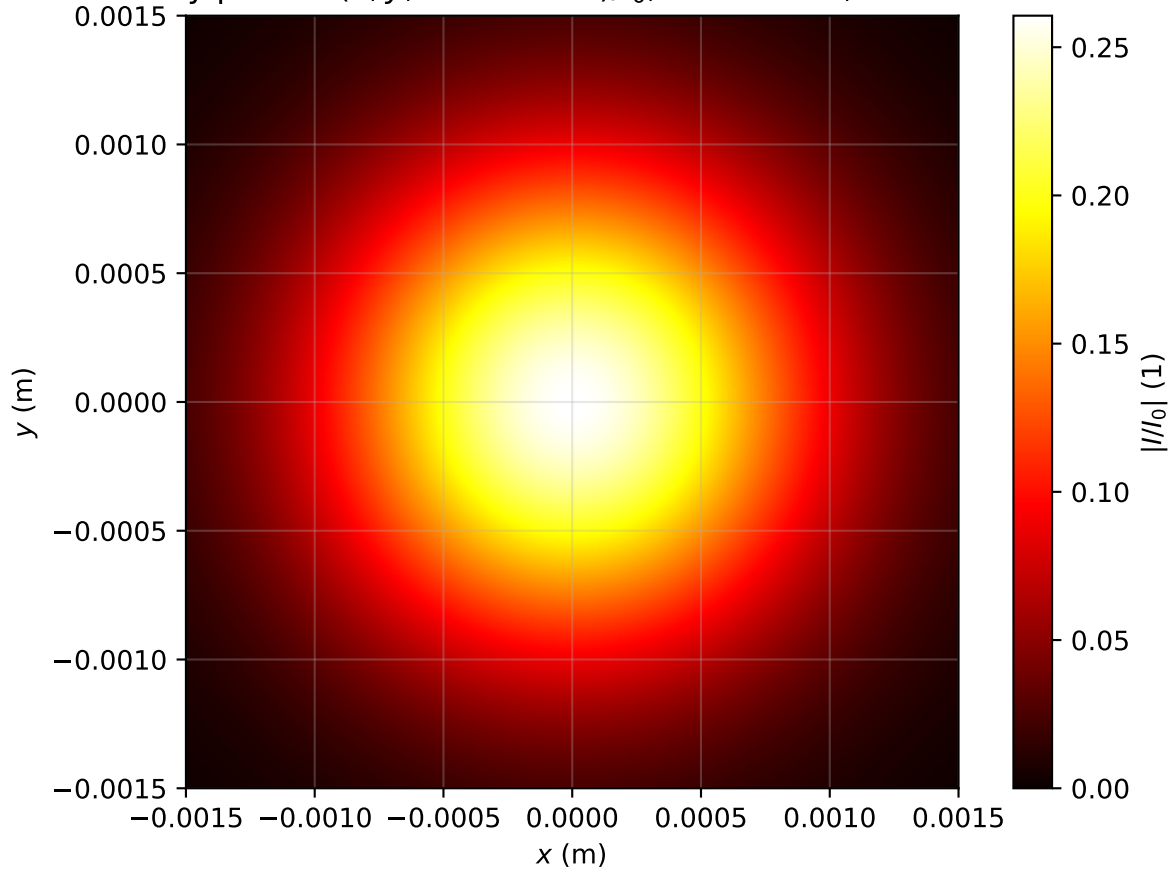
Intensity profile I(x, y, z = 3.582m)/I_0 , P_{in}=0.1P_{cr} , artificial time
